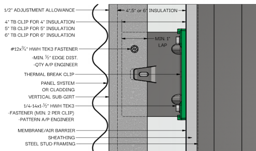
VERTICAL SUB-GIRT
