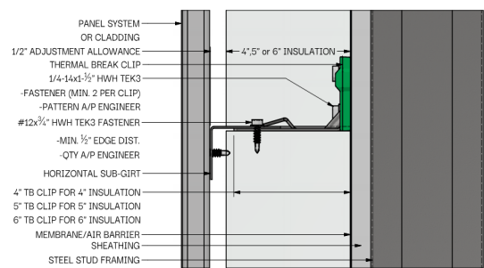
HORIZONTAL SUB-GIRT
